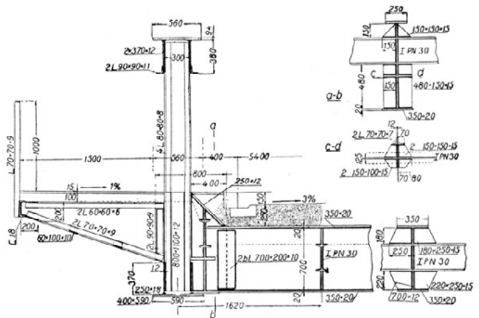
Fig. 2. Cross-section of the span of the bridge in Maurzyce [1]
