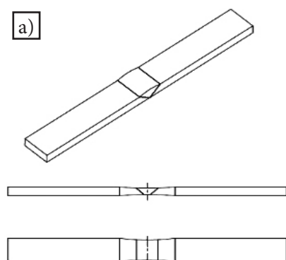
Fig. 6. Stages of the preparation of a specimen used in tensile tests of butt welded joints (a), present specimens (b)
