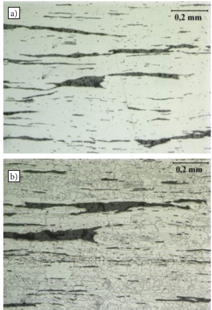
Fig. 11. Non-metallic inclusions in the form of slag and large sulphides arranged in bands in accordance with the direction of plastic working; unetched (a) and chemically etched in Nital (5 % HNO3) (b) [16]
