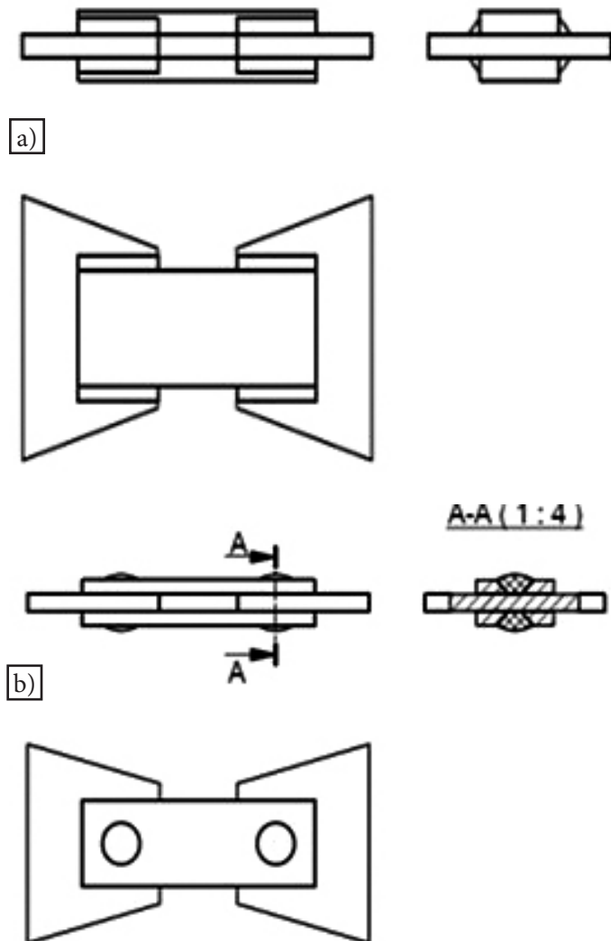
Fig. 9. Stages of the preparation of specimens used in the shearing test of welded joints: fillet welds (a) and plug welds (b)
