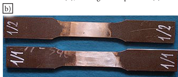
Fig. 6. Stages of the preparation of a specimen used in tensile tests of butt welded joints (a), present specimens (b)
