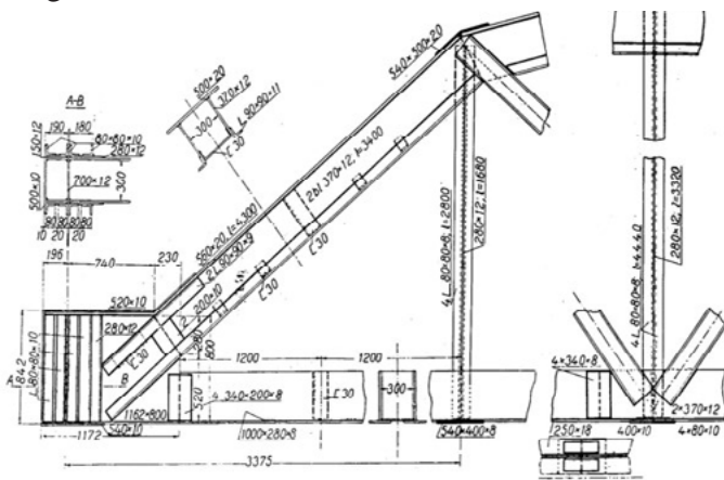
Fig. 1. Side view of the structure of the truss girder of the main span of the bridge in Maurzyce [1]
