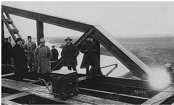
Fig. 5. Welding of a truss shoe; Professor S. Bryła (second from the left, wearing glasses) [13]
