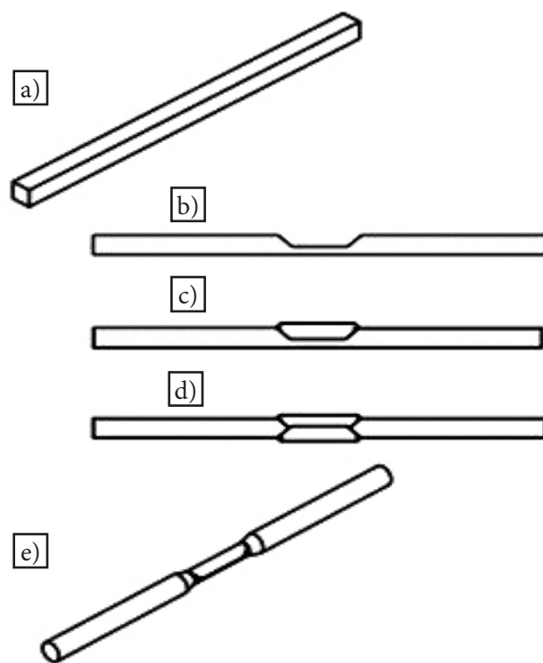
Fig. 8. Stages of the preparation of specimens used in the elongation of the weld in the static tensile test: cutting out the material (a), milling of the seat and the position of weld no. 1 (b, c), milling of the seat and the position of weld no. 2 (d), turning of the specimen (e)
