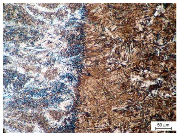
Fig. 7. Microstructure of the joint made of S355J2G3 steel using the local dry chamber method and arc welding with solid wire electrode; the view of the weld, fusion line and HAZ.
