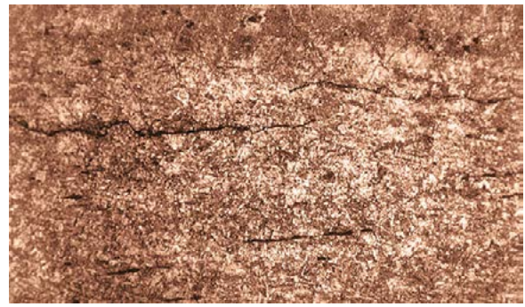
Fig. 6. Microstructure of the joint made of S420G2+M steel using the local dry chamber method and arc welding with solid wire electrode; numerous cracks in the joint HAZ. Mag. 200 \times .
