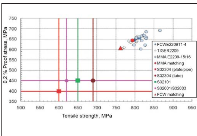
Fig. 10. Actual strength duplex weld metals compared to lean duplex base material requirements
