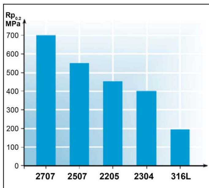
Fig. 2. Minimum proof strength
