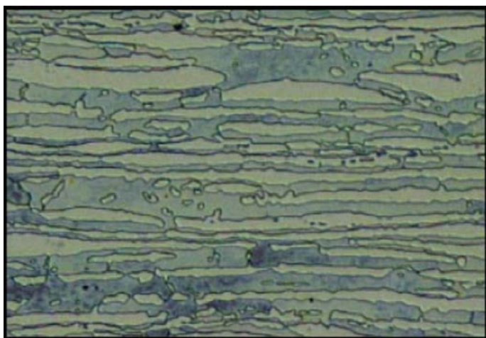
Fig. 1. Grade S32205 (Mag. 250x)
