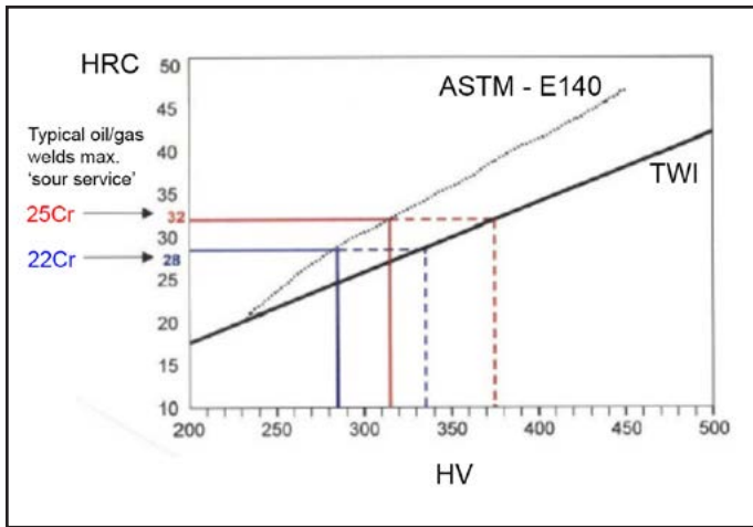
Fig 7. Correlation hardness H_V vs. H_{RC}
