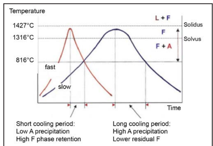
Fig. 6. Effect of cooling rate on ferrite content
