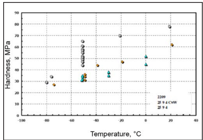
Fig 5. Transition curve all weld FCW deposits
