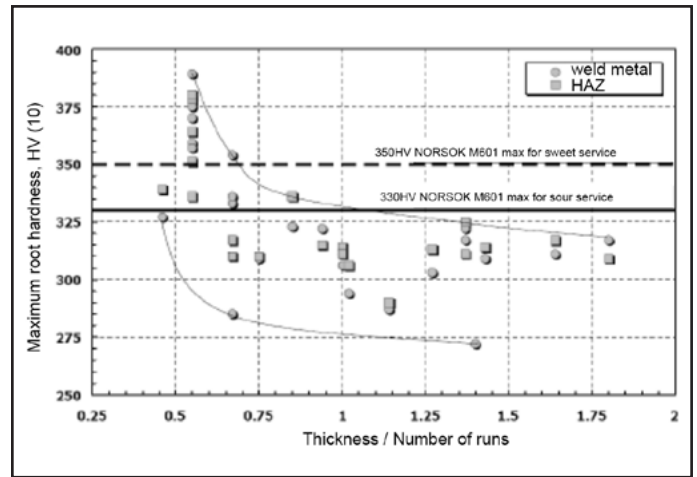
Fig 8. Effect of "thickness/runs" on hardness
