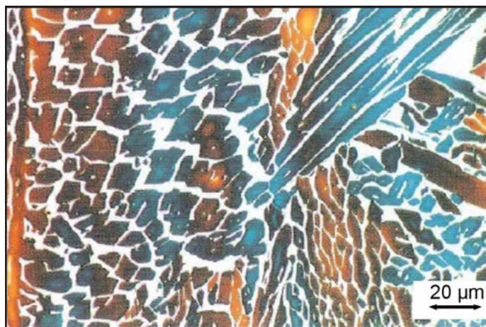
Fig. 3. Austenite in ferritic matrix (FN35)
